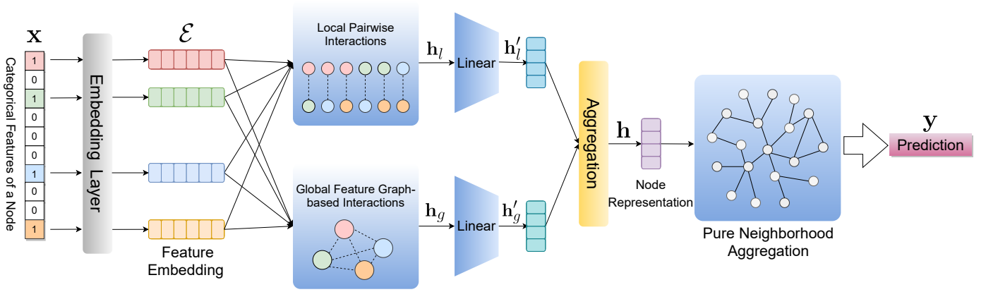
Fig. 1. The framework of CatGCN where an example node is taken to demonstrate the procedure of computing the initial node representation. Here, the feature number ( d ), embedding size ( D ), and prediction classes ( C ) are set as 10, 6, and 4, respectively.
