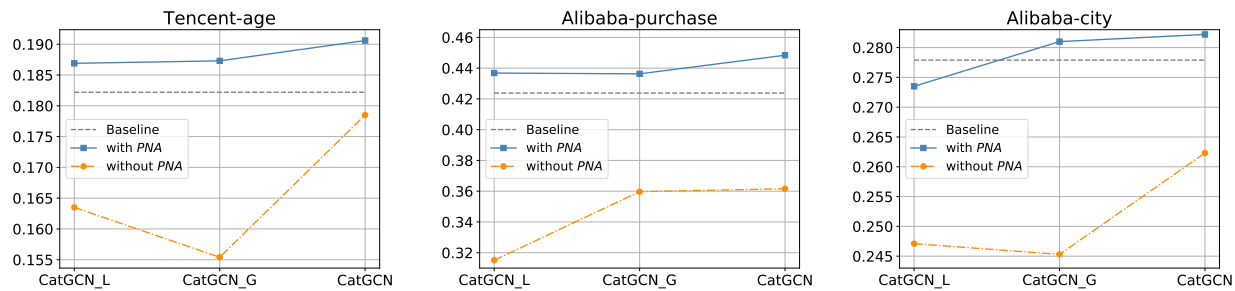
Fig. 4. Impacts of pure neighborhood aggregation.
