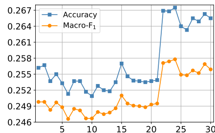
Fig. 5. Performance of CatGCN_G ( L=1 ) as adjusting the probe coefficient \rho on Alibaba-city task.
